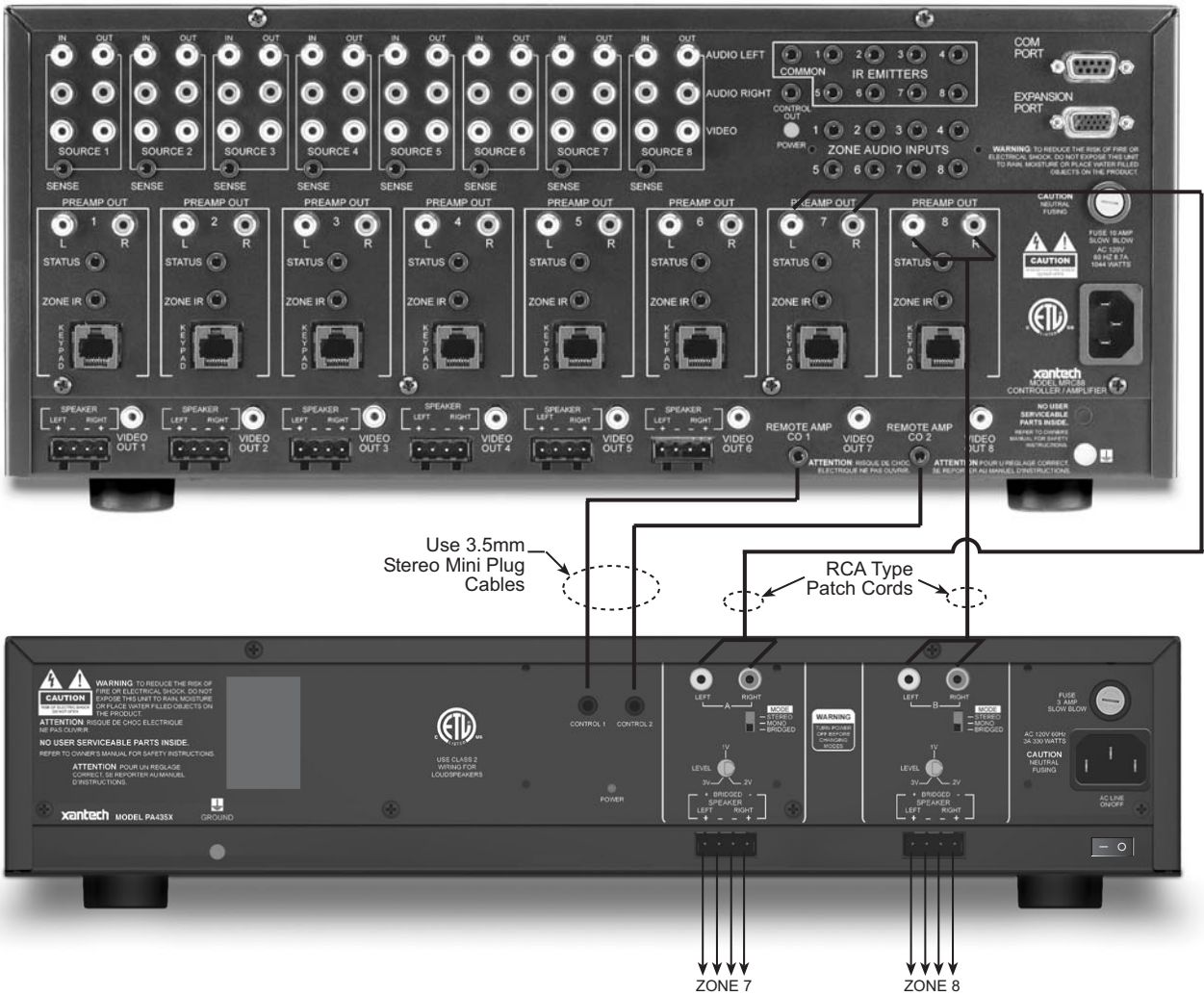
Figure 9: Interfacing the PA435X with an MRC88 Zones 7 & 8
