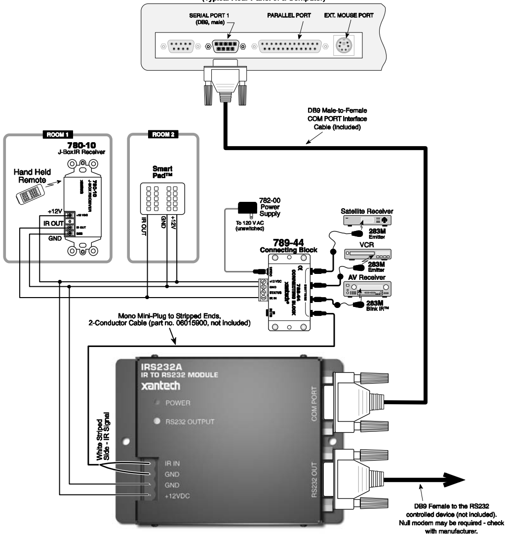
Figure 1 – Typical System Configuration with Programming Hardware Connections
