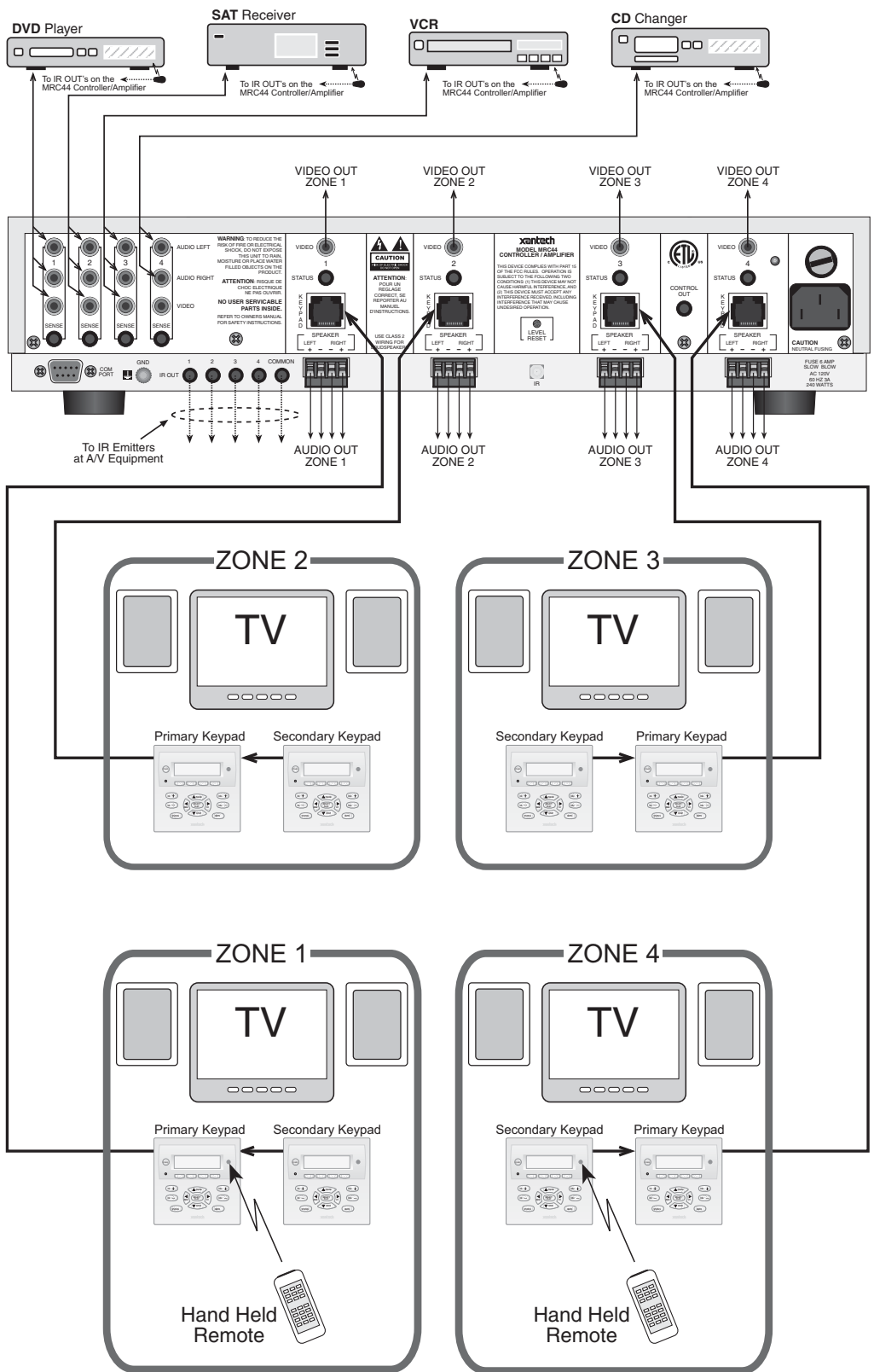
Figure 13 –Typical MRC44 System
